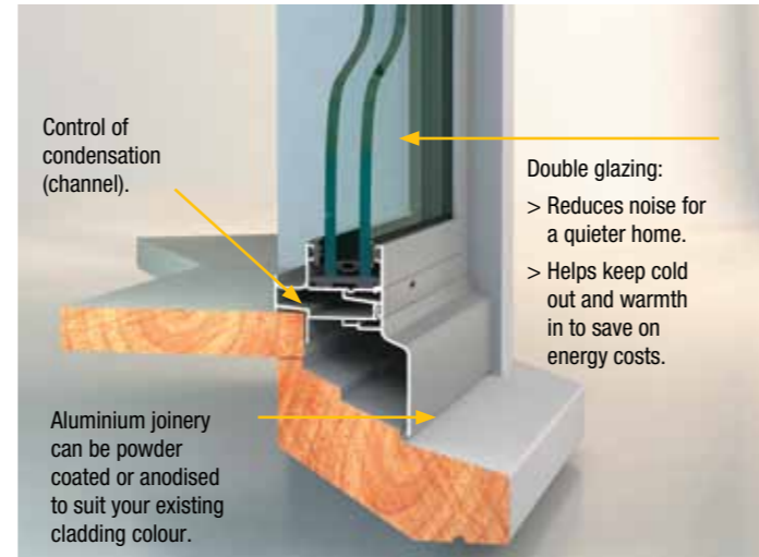
Close Up Insert Window Sill Detail
